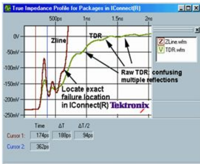
Serial data network analysis
