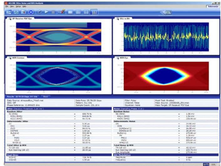
Jitter, noise and BER analysis
