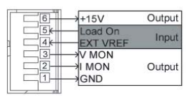
Pin Assignment for the Channel Control Connectors
