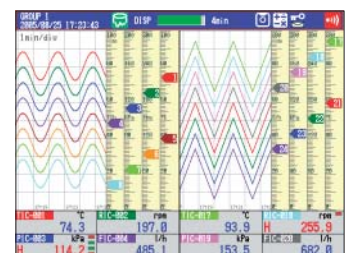
– Horizontally Divided Trend Display –
